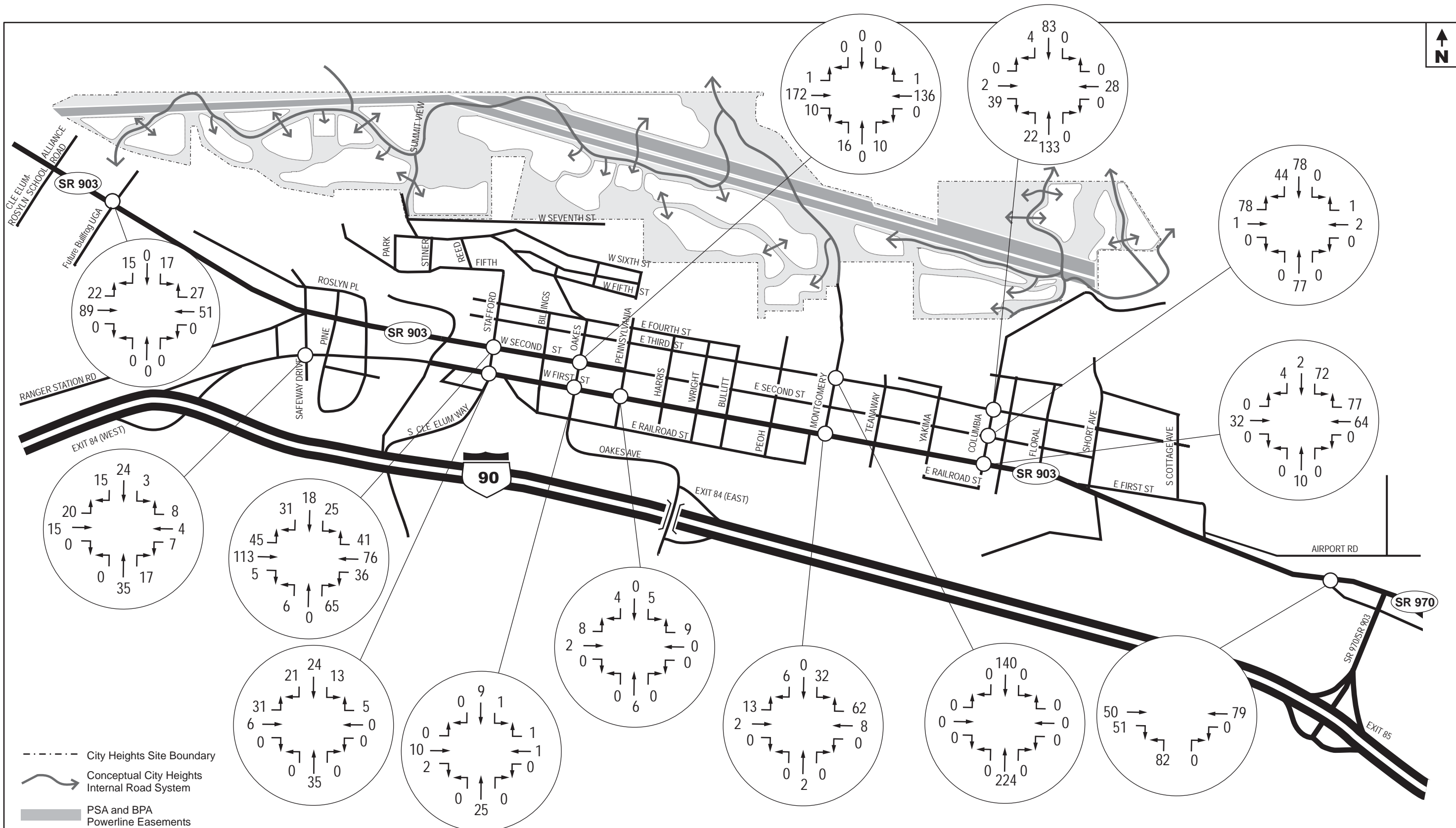
Figure 3.16-4 Alternative 1 PM Peak Hour Trips
