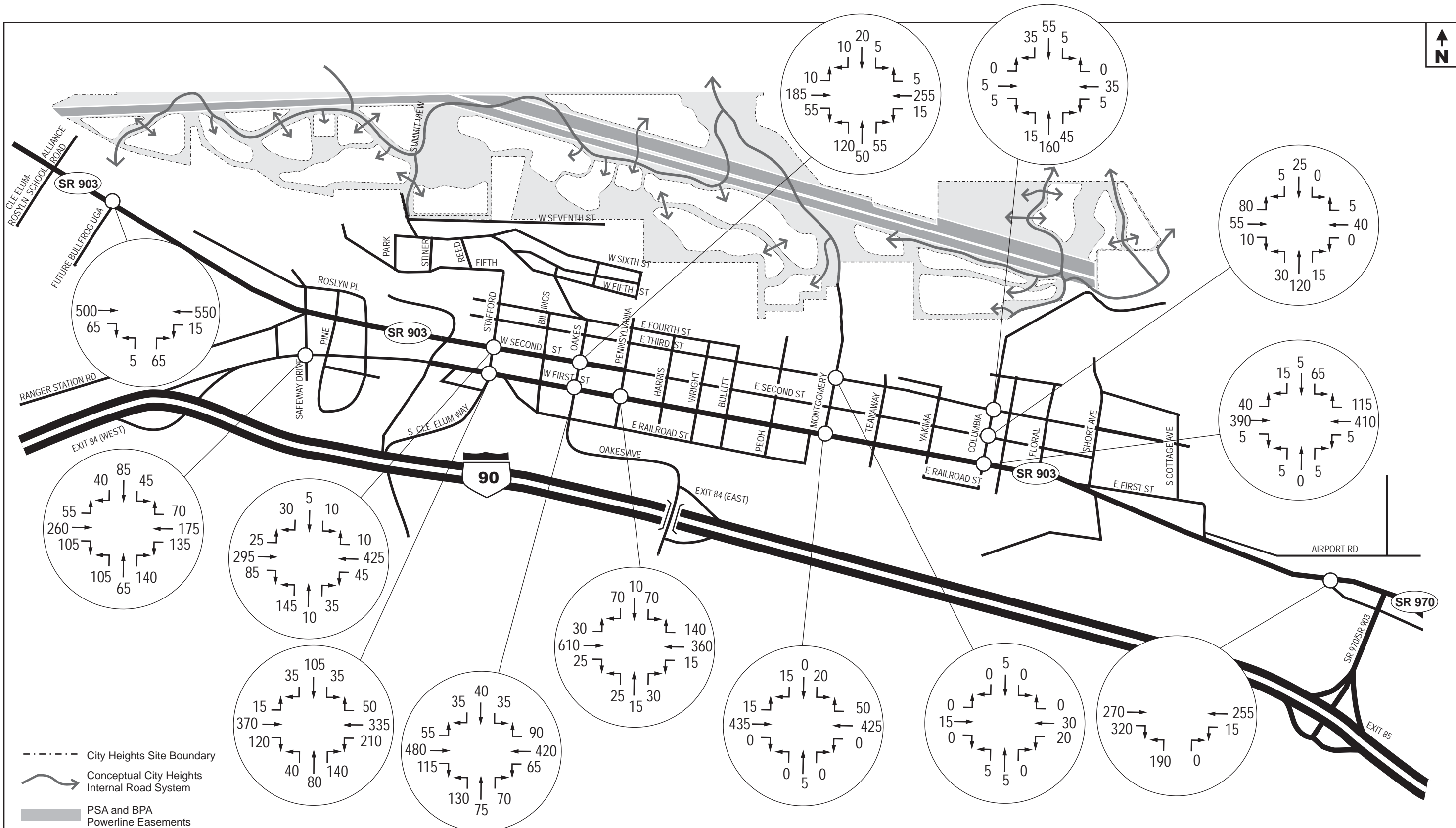
Figure 3.16-3 Future Without Project (Year 2022) PM Peak Hour Traffic Volumes
