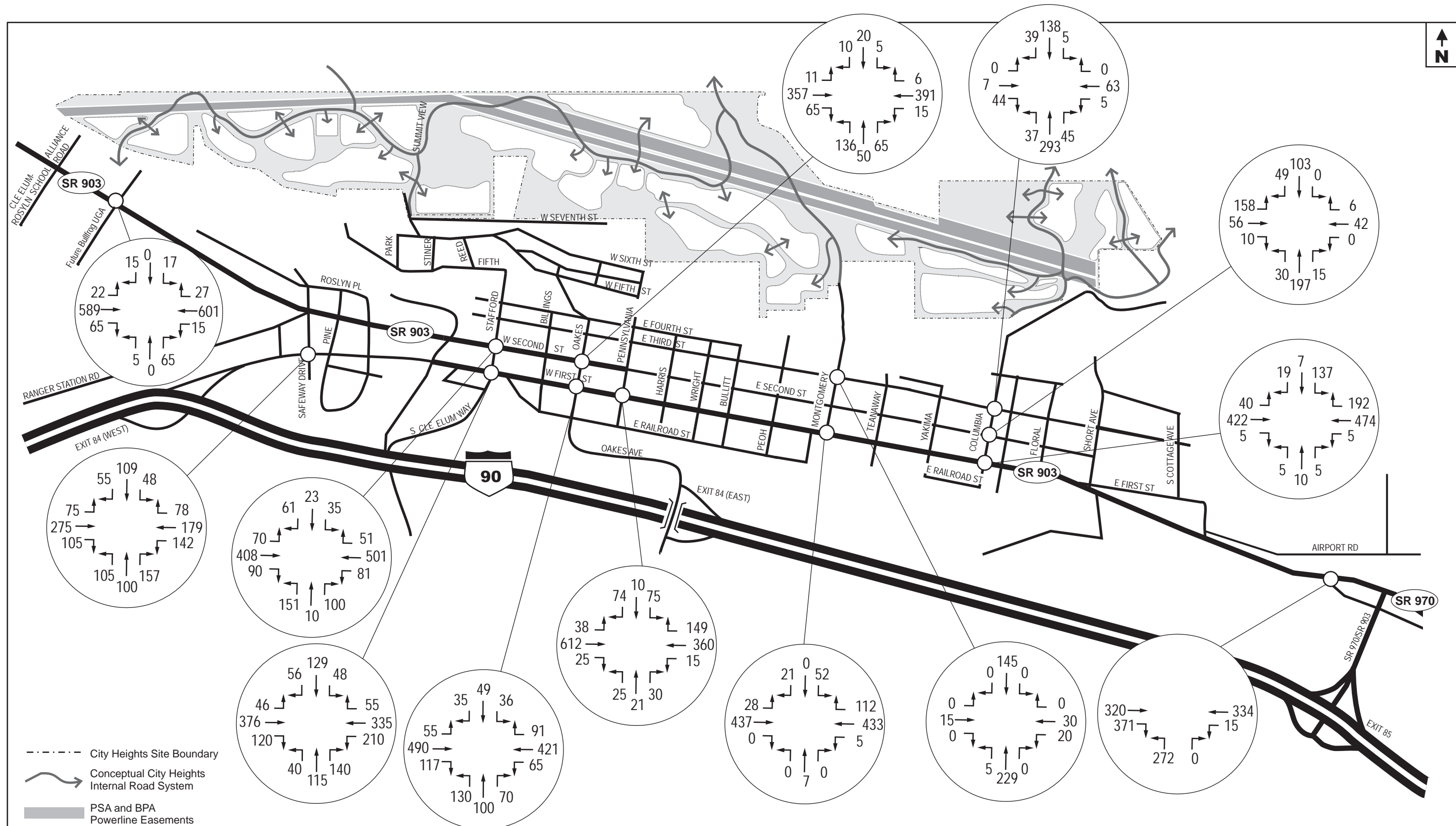
Figure 3.16-5 Future With Alternative 1 (Year 2022) PM Peak Hour Traffic Volumes
